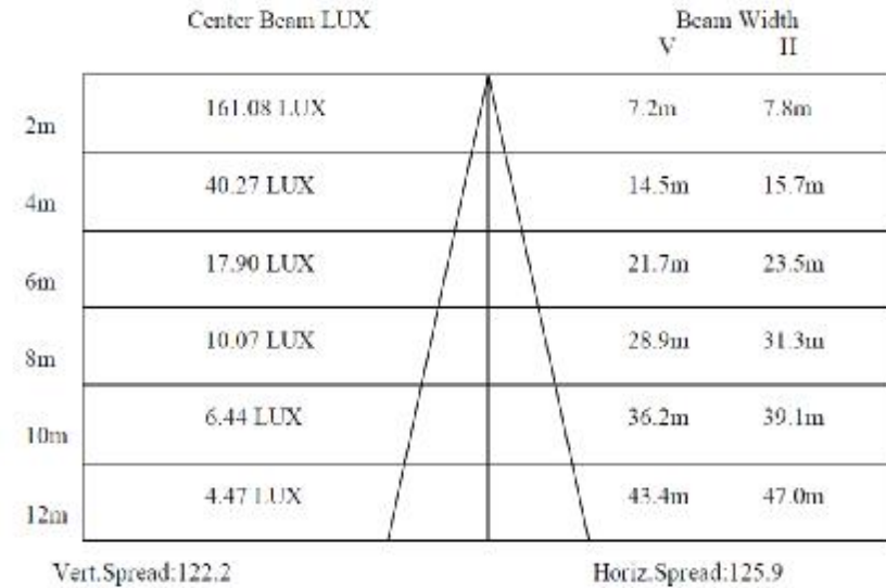
Illumination Drawing(High 4 meters)
